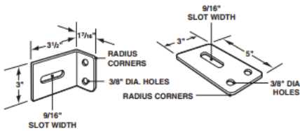
ANGLE AND FLAT MOUNTING BRACKETS
